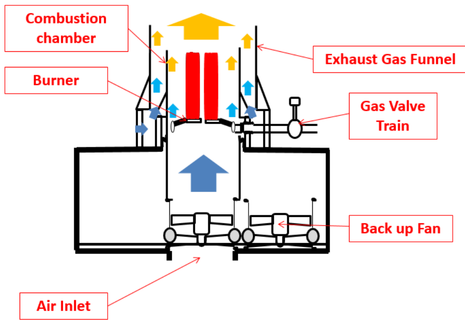
ECOFLARE main Components and architecture (Patent pending)
