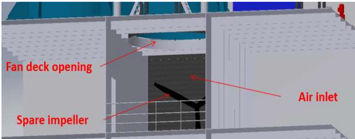
Air inlet arrangement
