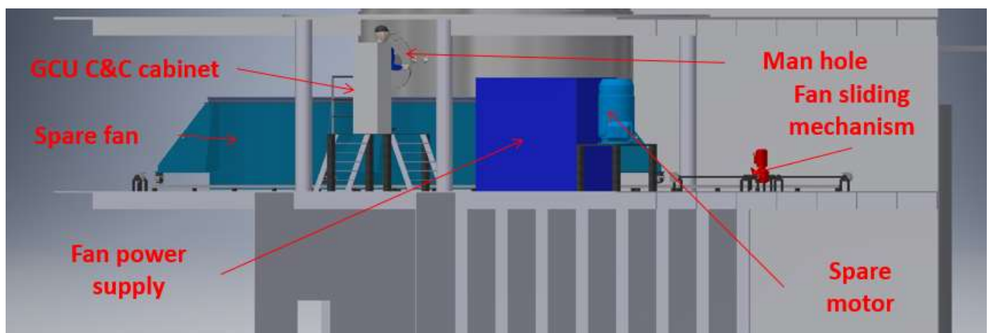
Fan deck arrangement
