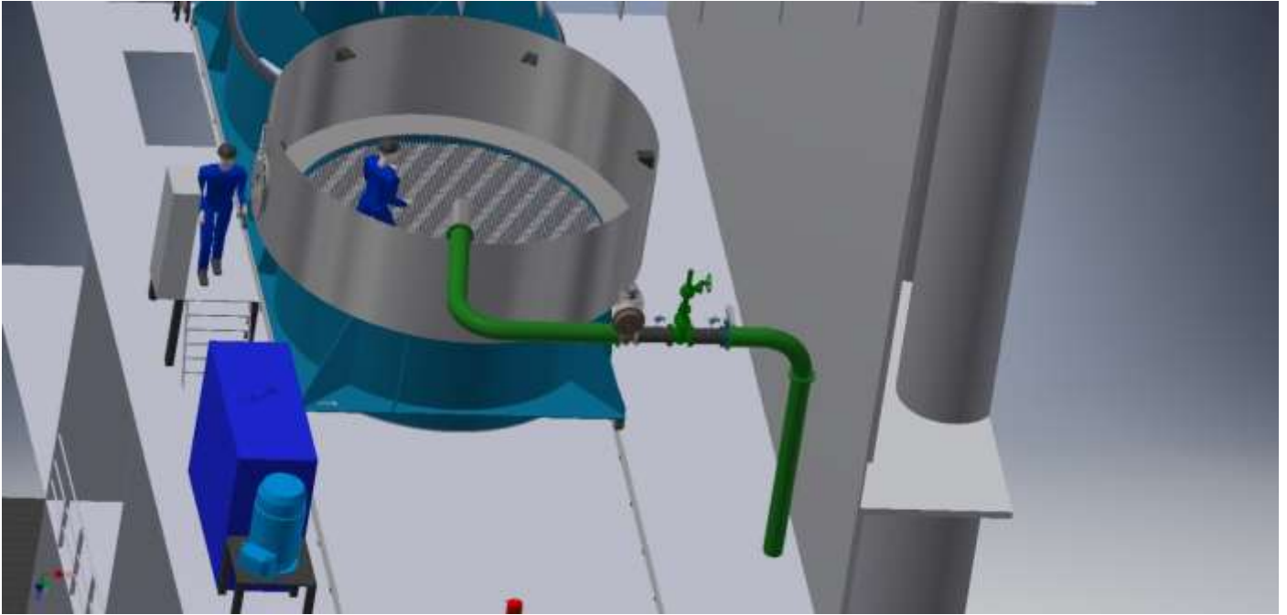
Removable fan grid platform for burner and combustion chamber maintenance operations
