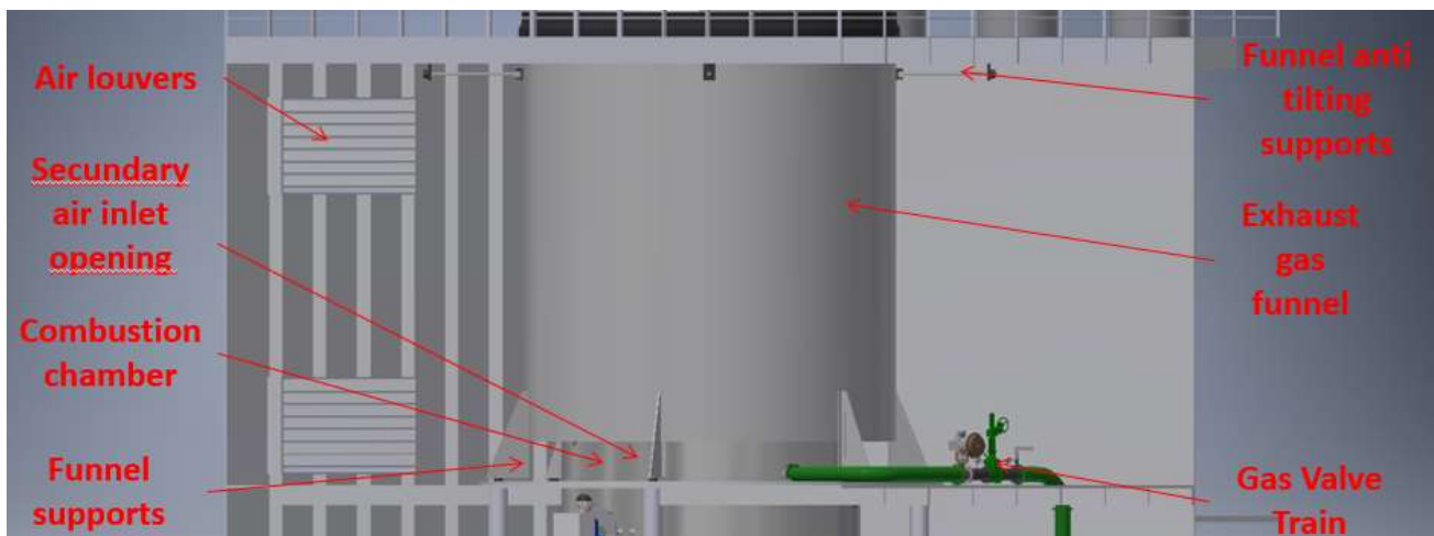
Burner deck arrangement
