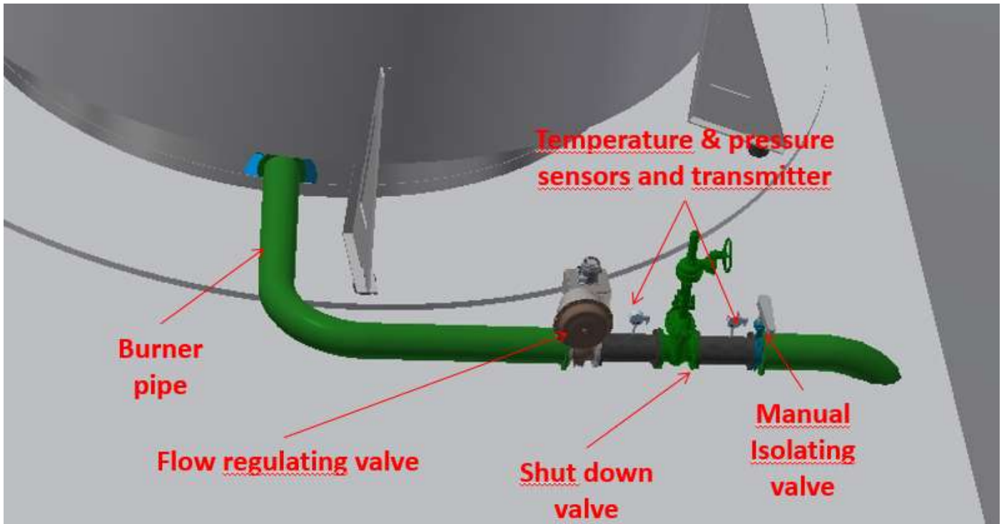
Gas valves train
